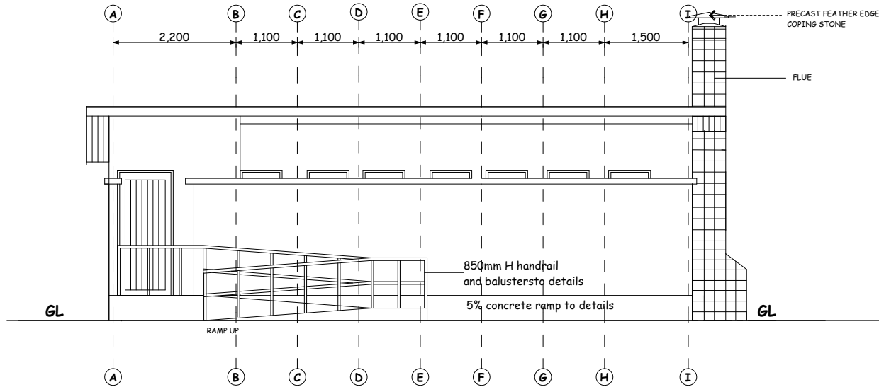
FRONT ELEVATION
