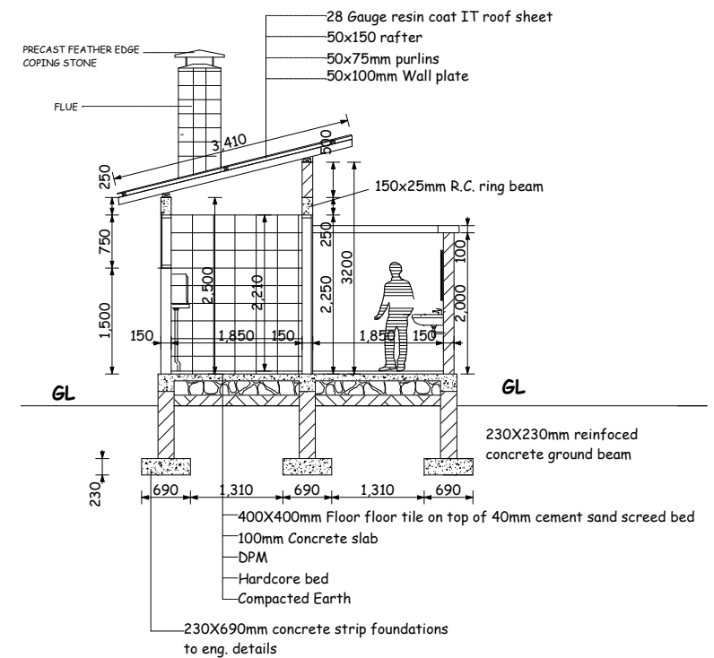
TYPICAL SECTION
