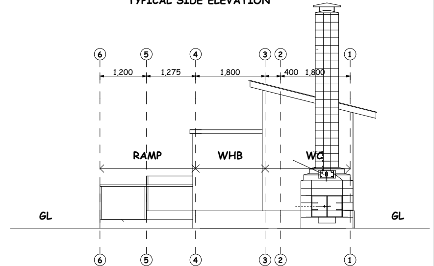
TYPICAL SIDE ELEVATION
