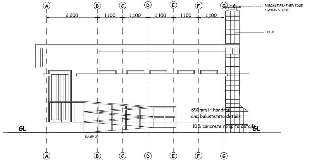
FRONT ELEVATION
